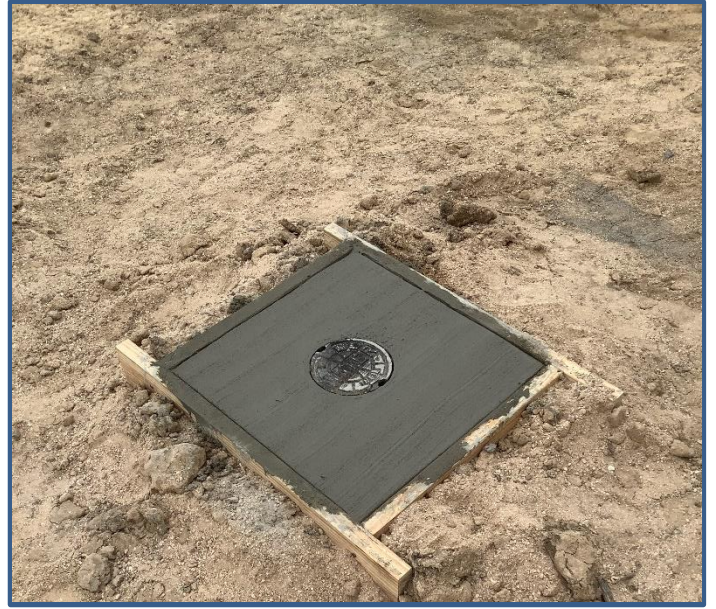
Cleanout Installed and Concrete poured around
